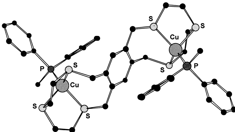
Fig. 1. The X-ray structure of the cation anti -[Cu 2 L(PPh 2 Me) 2 ] 2+ [L=(17)] [18].
