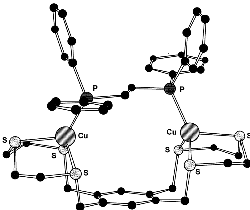
Fig. 2. The X-ray structure of the cation syn -[Cu 2 L(μ-PPh 2 CH 2 CH 2 PPh 2 )] 2+ [L=(17)] [28].
