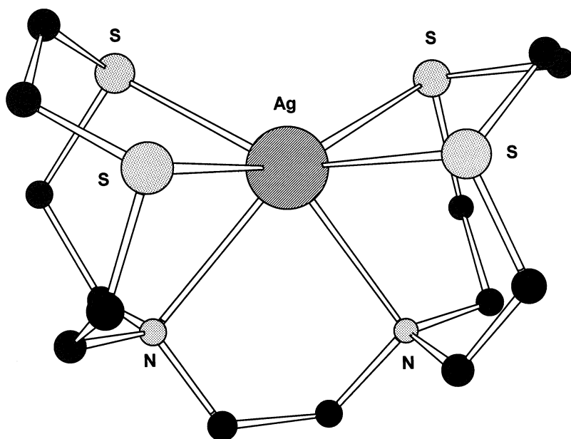
Fig. 3. The X-ray structure of the cation [\text{AgL}]^+ [ \text{L}=(21) ] [23].
