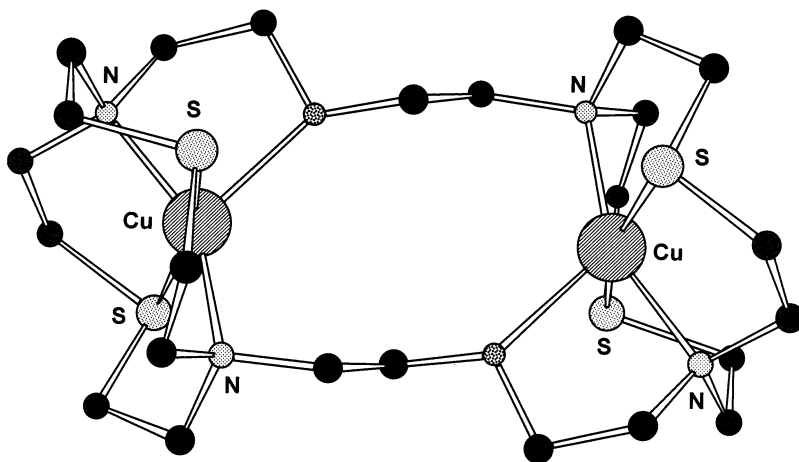
Fig. 4. The X-ray structure of the cation [Cu 2 L] 4+ [L = (22)] [27].
