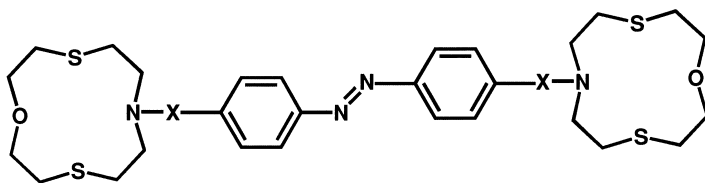
(19) ( X = \text{CH}_2 or \text{CO} )
